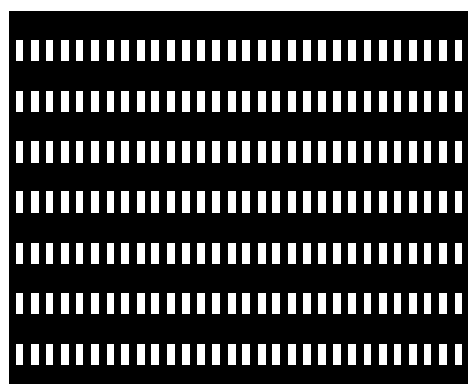
Nr. 4130 mm hole width b x h 0,9 x 2,5 pitch horizontal 1,8 pitch vertical 6,0 opening 21 %
